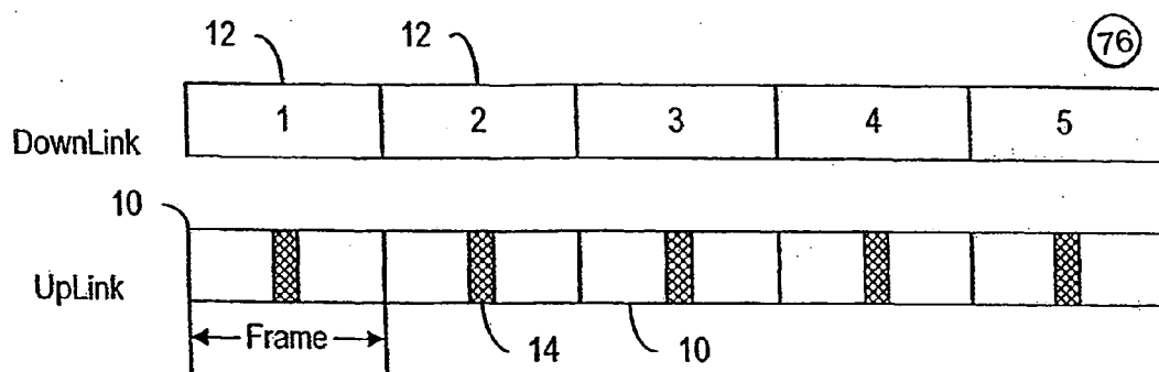
Figure 1 Uplink and DownLink Frames
