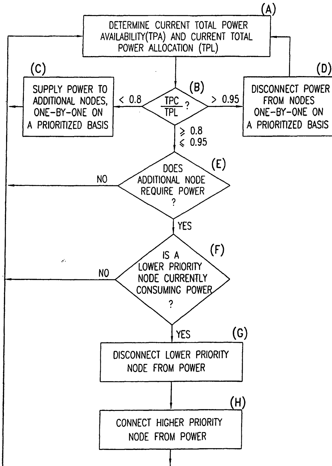
FIG. 23A VOLUNTARY POWER MANAGEMENT FULL FUNCTIONALITY OR NO FUNCTIONALITY
