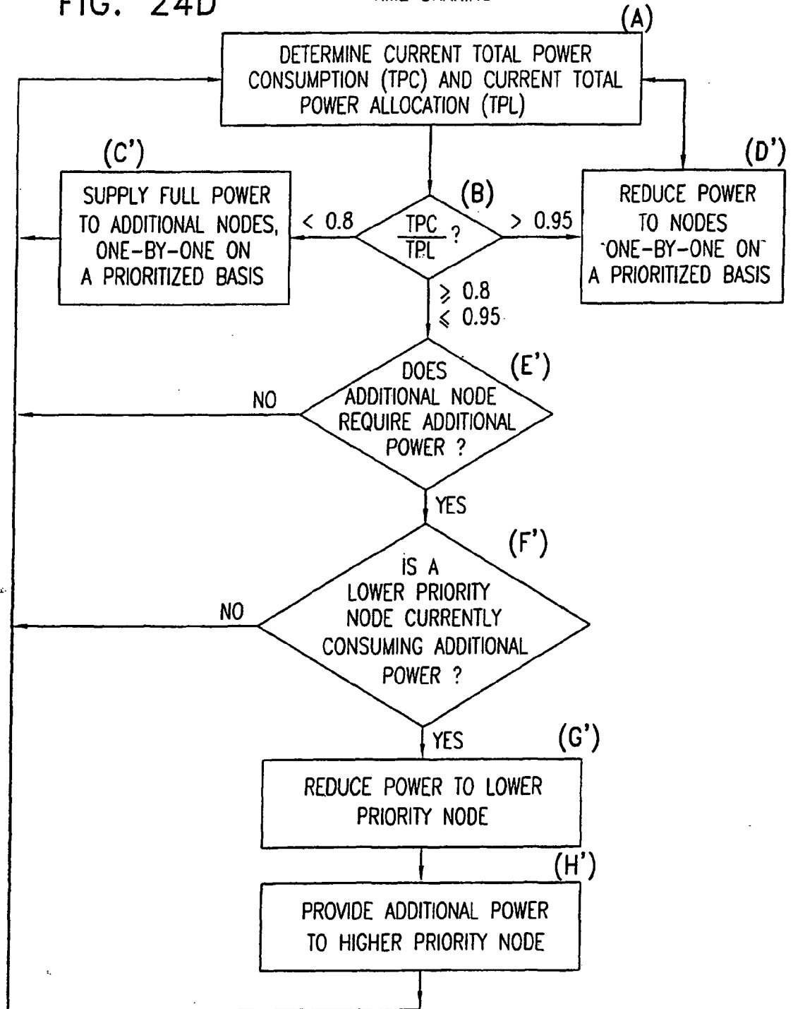
FIG. 24D VOLUNTARY POWER MANAGEMENT FULL FUNCTIONALITY OR REDUCED FUNCTIONALITY TIME SHARING
