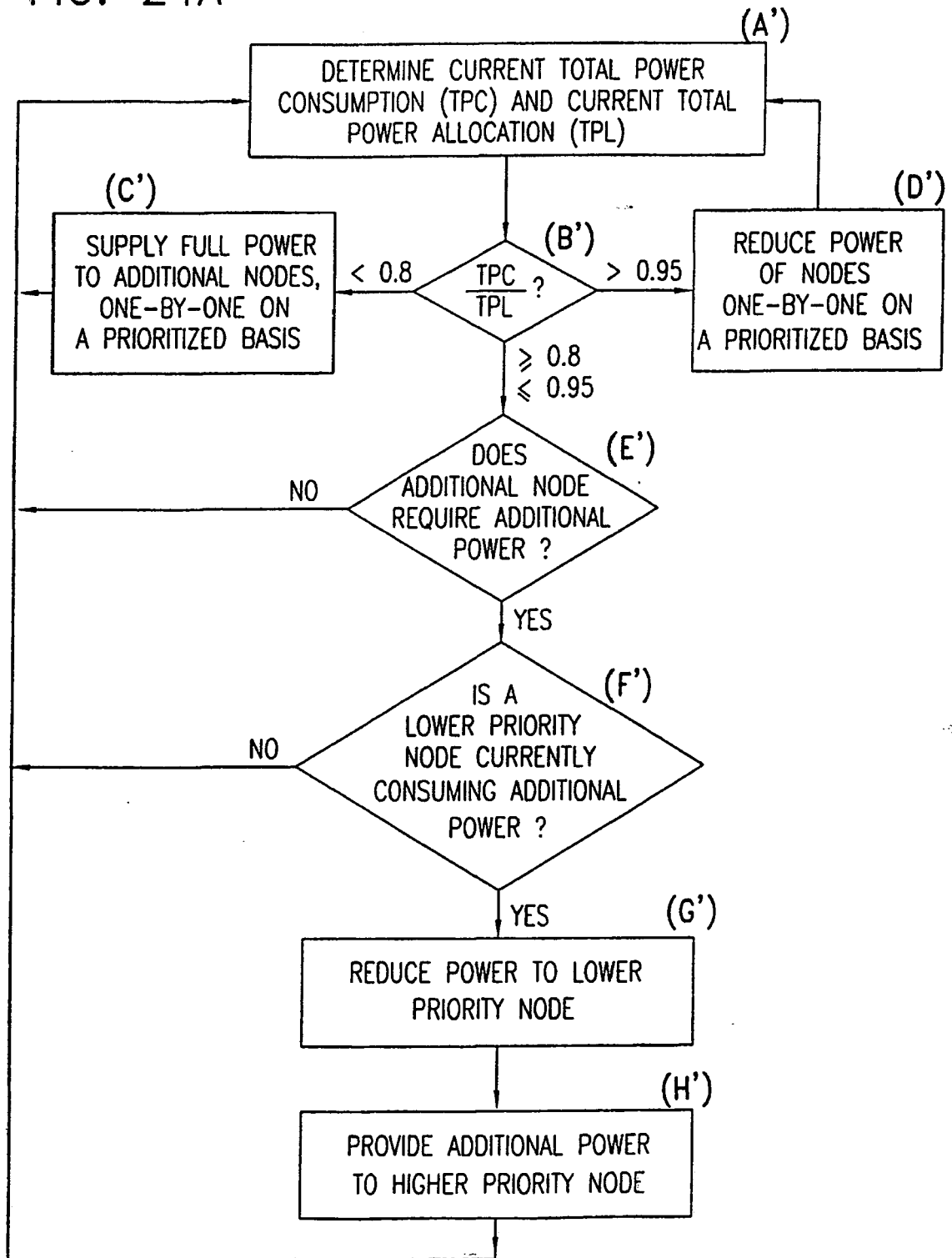
FIG. 24A VOLUNTARY POWER MANAGEMENT FULL FUNCTIONALITY OR REDUCED FUNCTIONALITY
