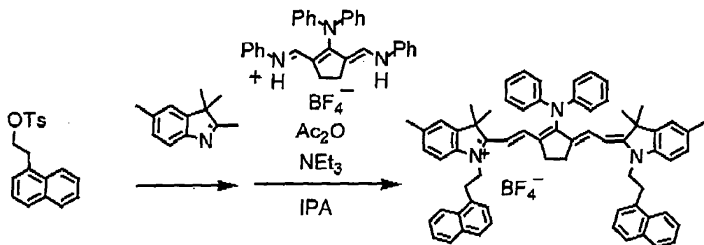
Infrared Absorbing Agent (1)
