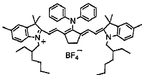
Infrared absorbing agent (7)
