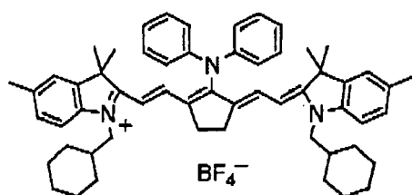
Infrared absorbing agent (8)
