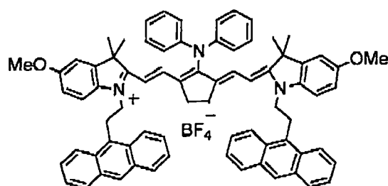
Infrared absorbing agent (9)
