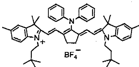
Infrared absorbing agent (6)
