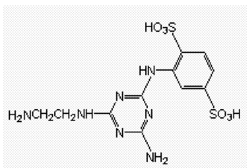
Compound (4)
