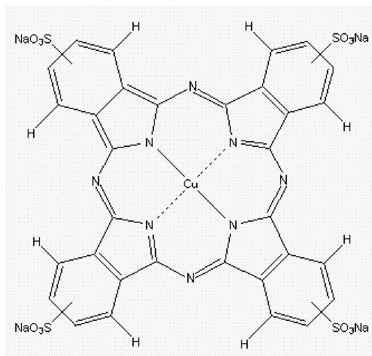
Compound (2)
