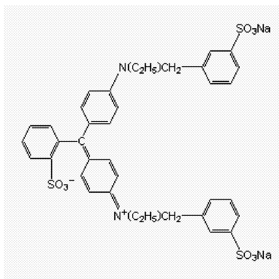
Compound (1)
