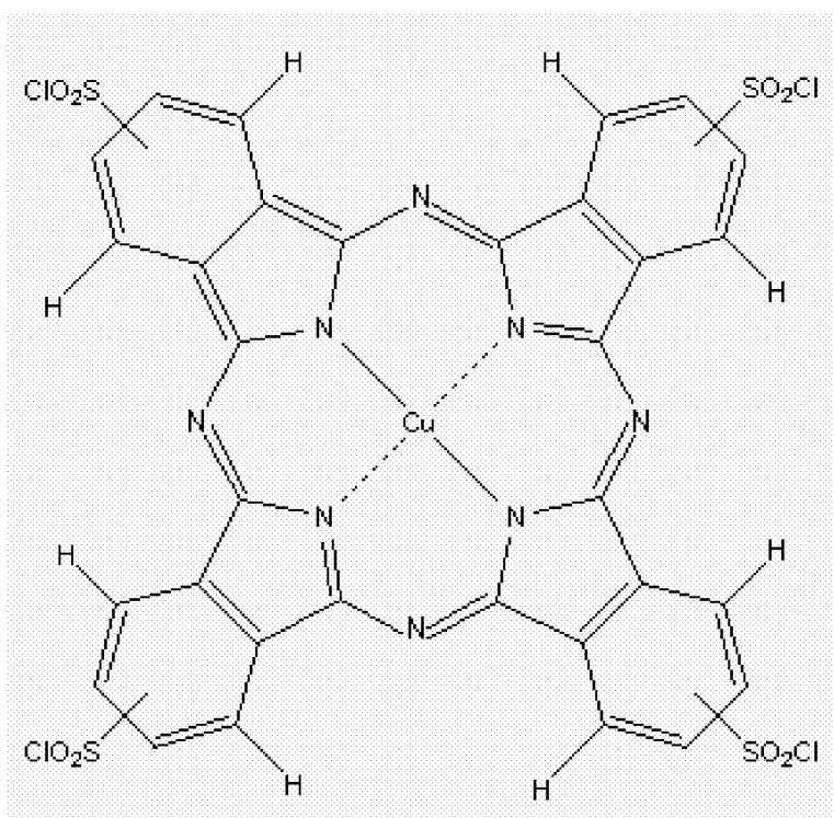
Compound (3)
