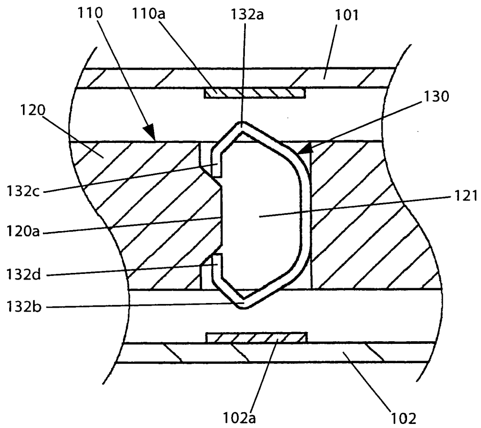
Fig. 6A Prior Art
