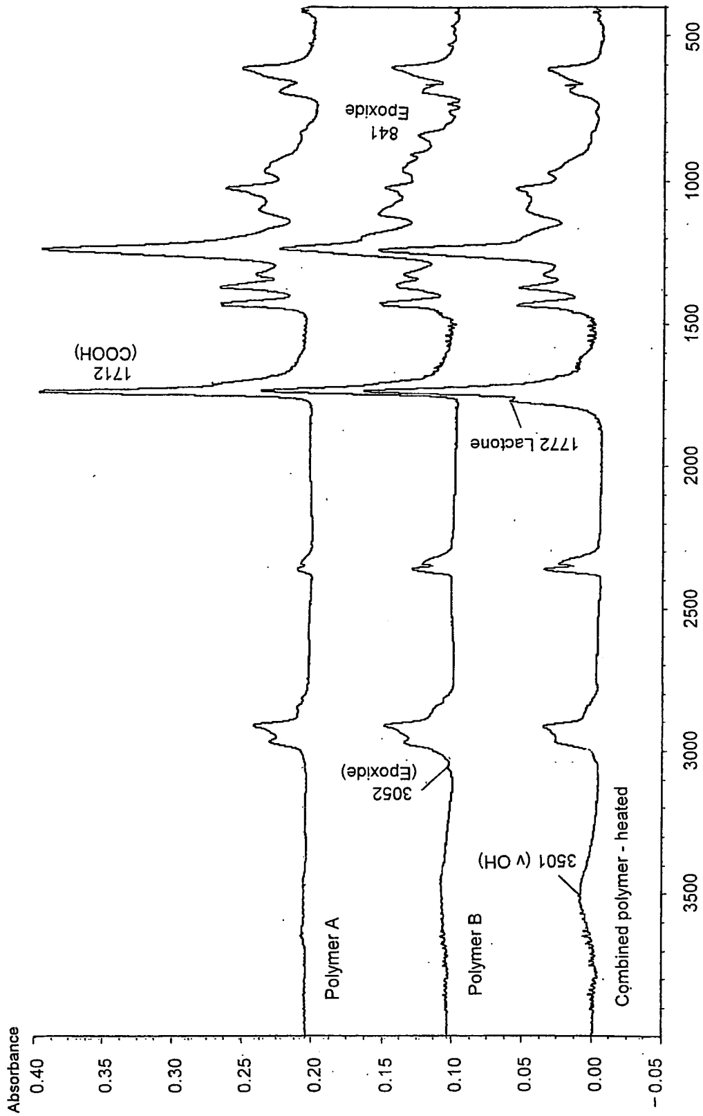
Wavenumbers (cm-1)
