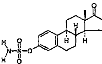
oestrone-3-sulphamate (EMATE)
