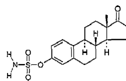
oestrone-3-sulphamate (EMATE)
