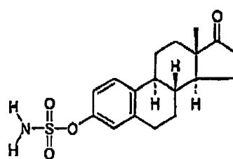
oestrone-3-sulphamate (EMATE)
