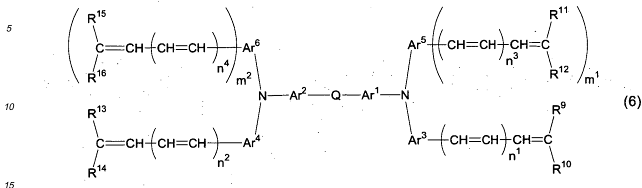
[Chemical formula 25]
