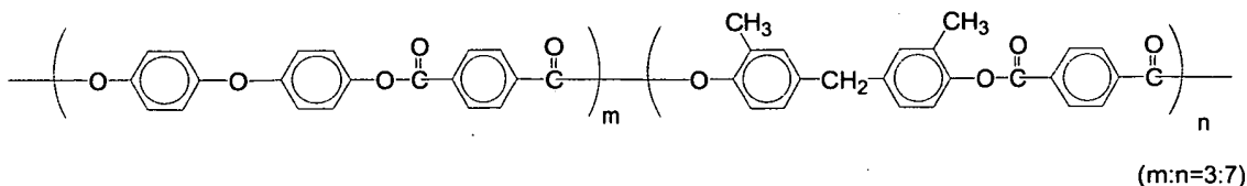
[Chemical formula 44]
