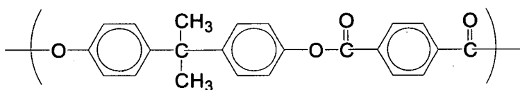
[Chemical formula 51]
