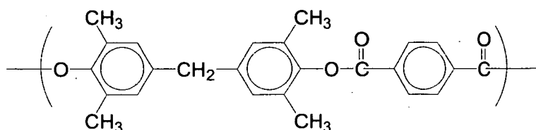
[Chemical formula 41]
