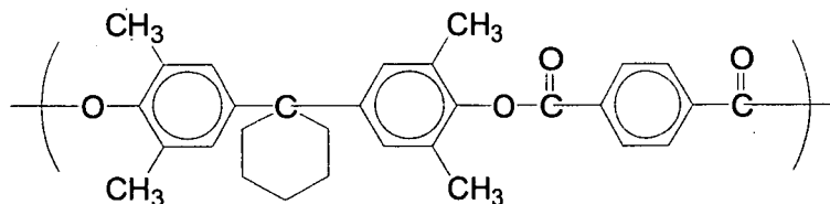
[Chemical formula 43]
