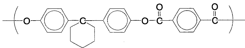
[Chemical formula 49]
