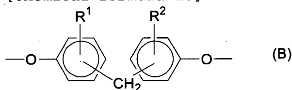
[Chemical formula 15]
