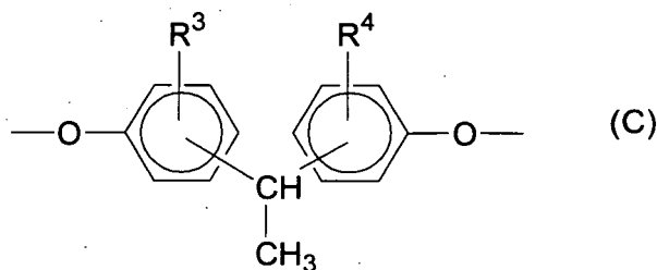
[Chemical formula 17]
