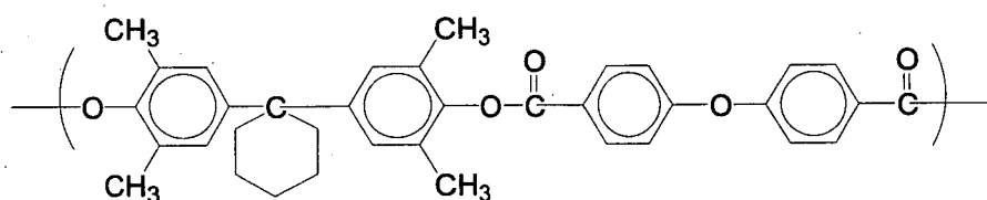
[Chemical formula 42]
