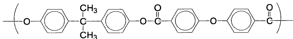
[Chemical formula 50]
