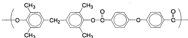
[Chemical formula 40]
