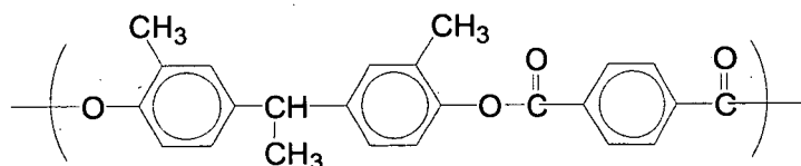
[Chemical formula 39]
