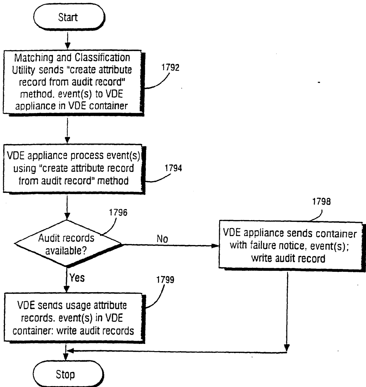
Fig. 44 Example steps for assembling usage audit records
