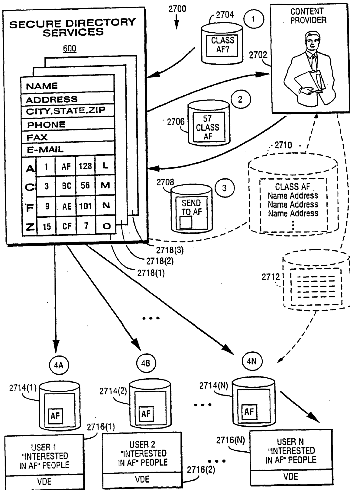
Fig. 52 Secure Directory Services
