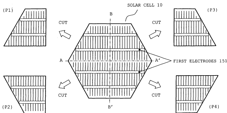
EXAMPLE OF CELL DIVISION
