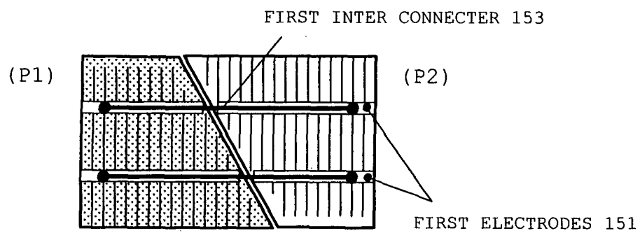
EXAMPLE OF UNIT CONFIGURATION
