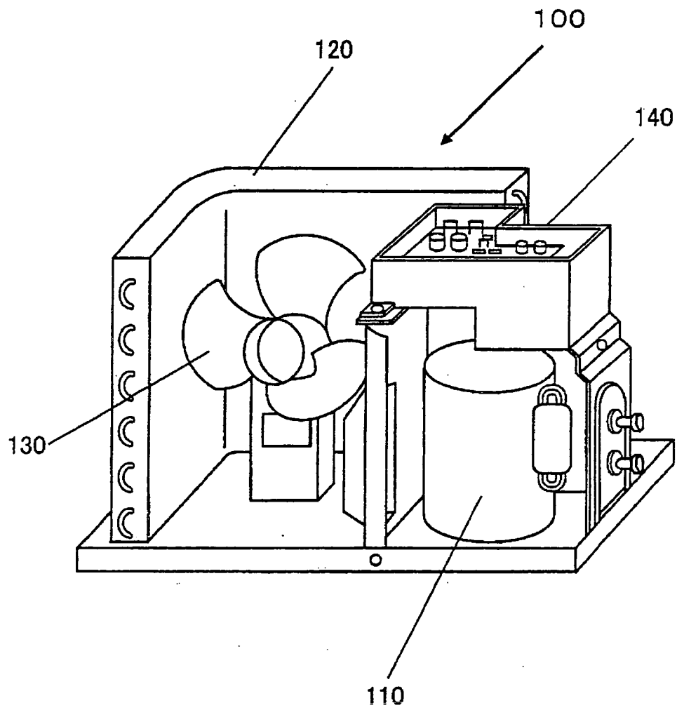
FIG. 6 (PRIOR ART)
