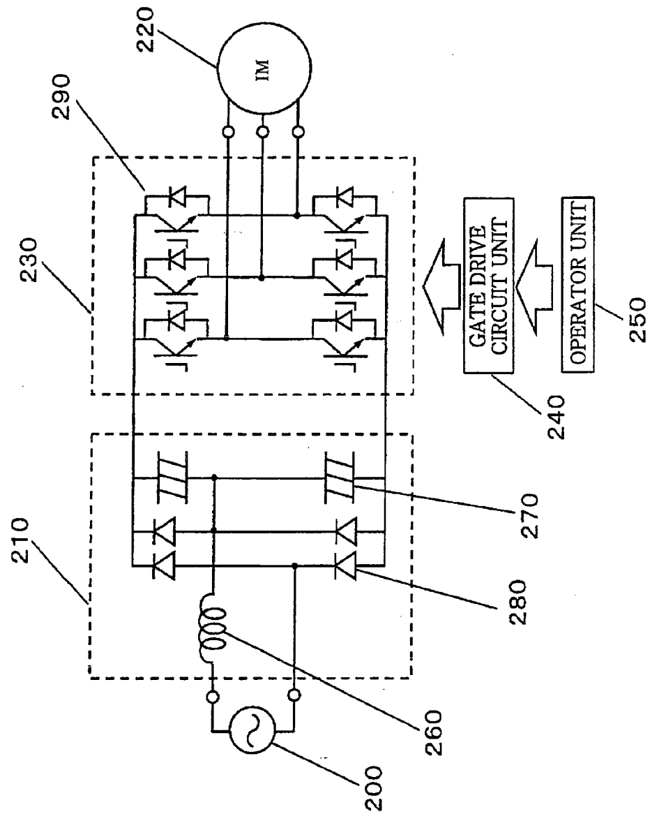
FIG. 7 (PRIOR ART)
