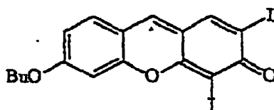
Di-iodobutoxy fluorone
