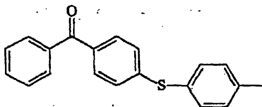
[4-(4-methylphenylthio)phenyl]phenylketone
