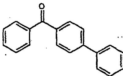
4-phenyl benzophenone
