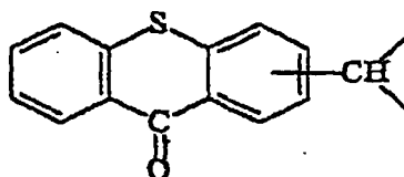
isopropyl thioxanthone
