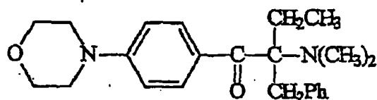
2-benzyl-2-N,N-dimethylamino-1-(4-morpholinophenyl)-1-butanone
