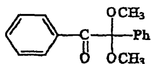
2,2-dimethoxy-2-phenyl acetophenone
