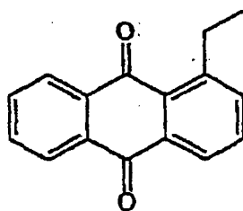
2-ethyl anthraquinone
