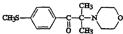
2-methyl-1-[4-(methylthio)phenyl]-2-morpholino propan-1-one
