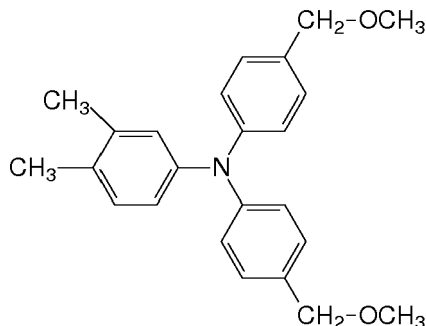
Compound (II)
