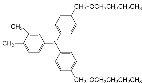
Compound (I)
