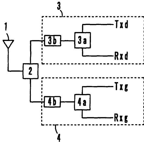
Fig. 19 PRIOR ART
