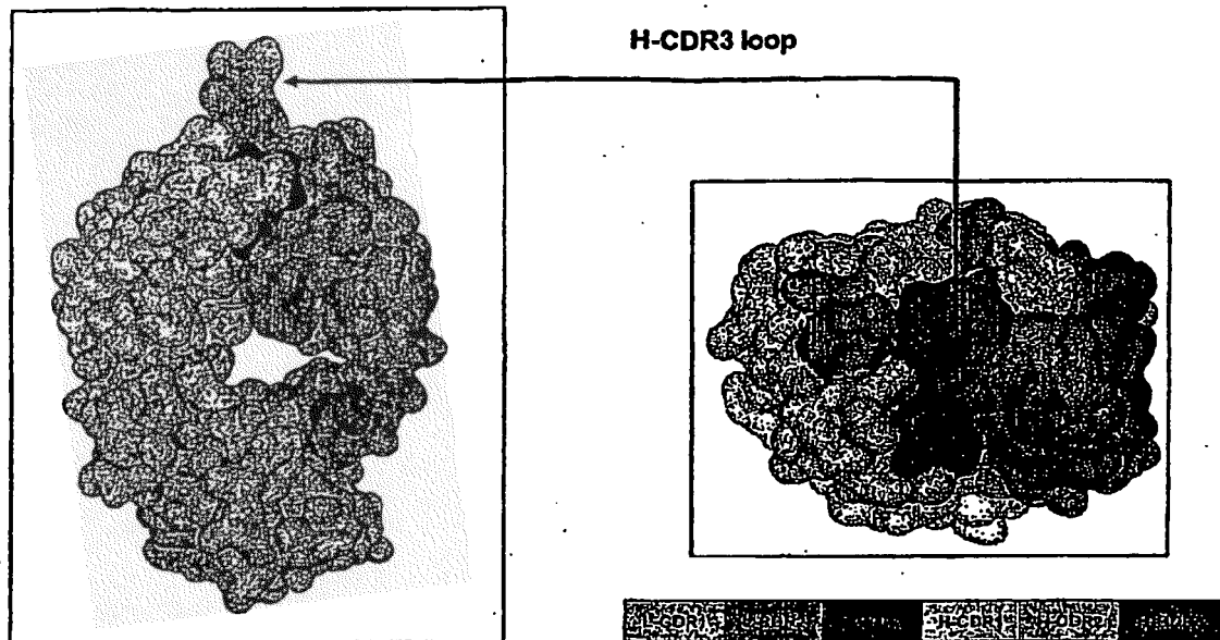
Figure 2. X-ray structure of AIN457 Fab, overall view
