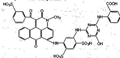
Exemplified compound 6
