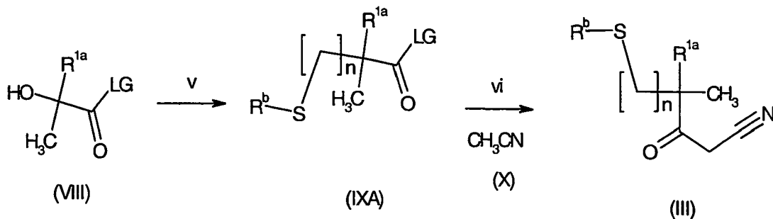
Scheme 3.1
