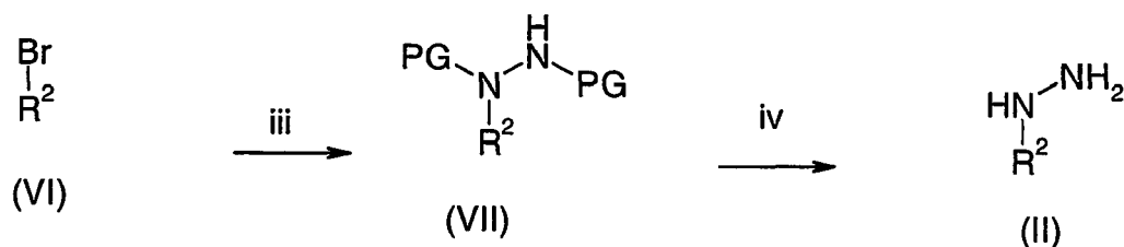
Scheme 2
