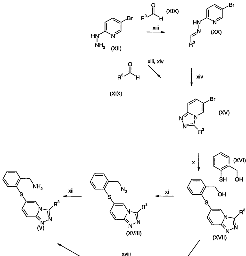
Scheme 5
