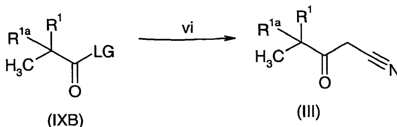
Scheme 3.2
