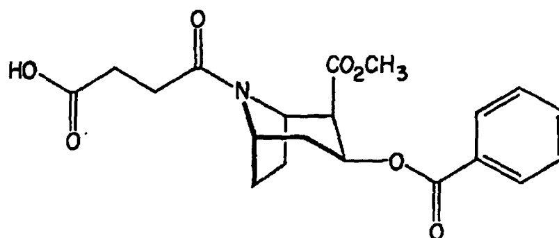
SUCCINYLATED NORCOCAINE
