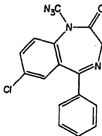
DIAZEPAM
