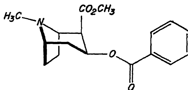
(-)-COCAINE
