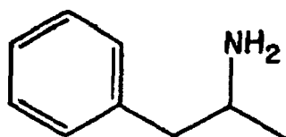
AMPHETAMINE
