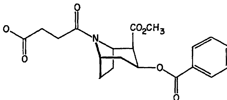
SUCCINYLATED NORCOCAINE
