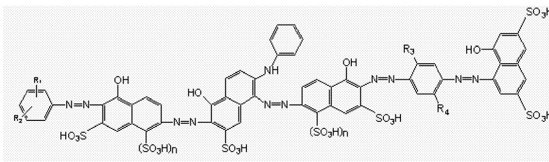
General formula (I)
