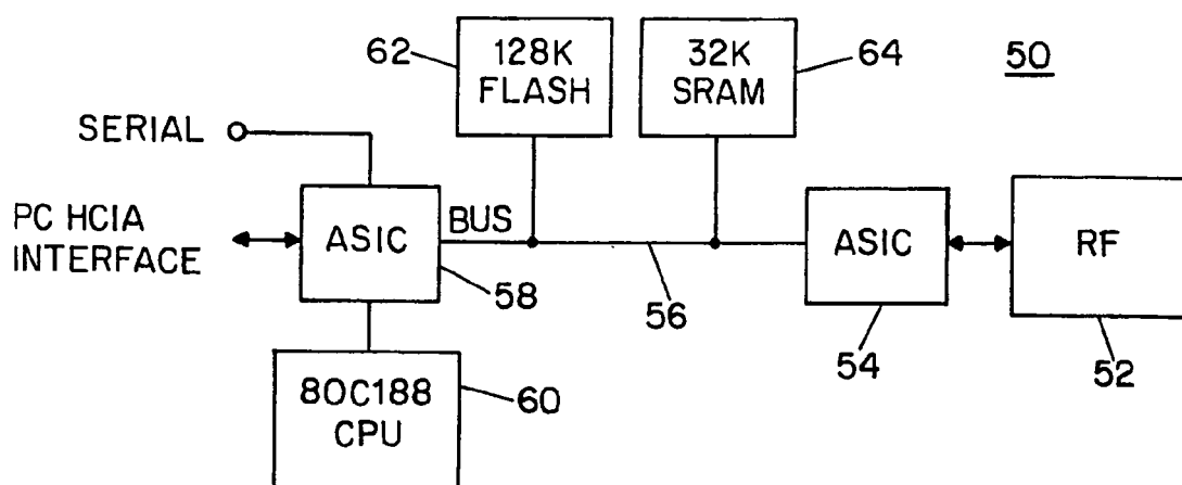
FIG. 8 PRIOR ART
