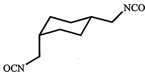
cis-1,4-bis(isocyanatomethyl)- cyclohexane Formula IV
