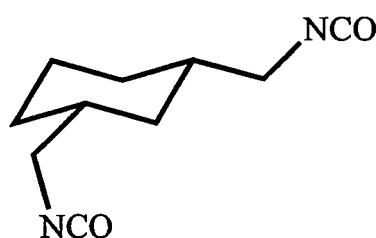
cis-1,3-bis(isocyanatomethyl)- cyclohexane Formula II
