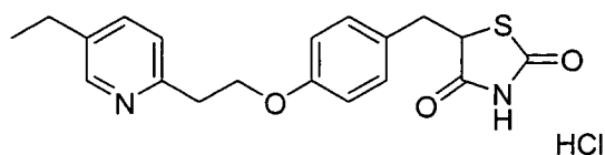
[Chemical formula 12]
