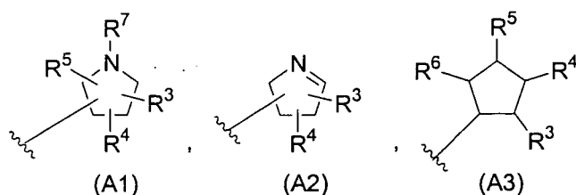
[Chemical formula 9]
