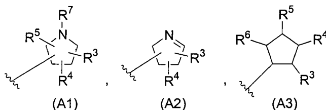
[Chemical formula 11]
