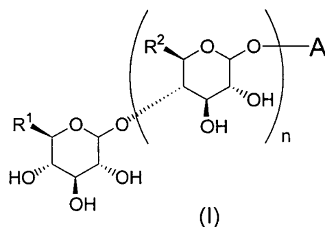
[Chemical formula 8]
