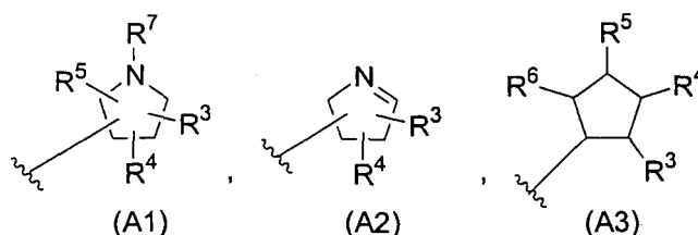
[Chemical formula 2]
