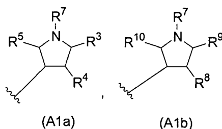
[Chemical formula 15]
