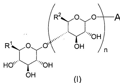
[Chemical formula 3]
