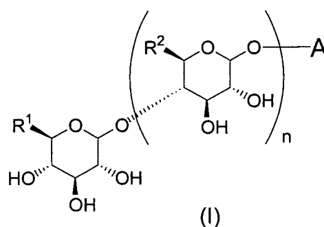
[Chemical formula 1]
