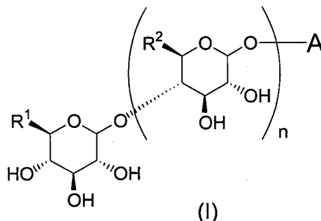
[Chemical formula 6]
