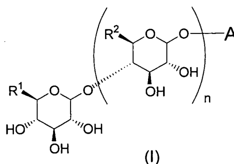
[Chemical formula 8]
