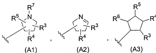
[Chemical formula 7]
