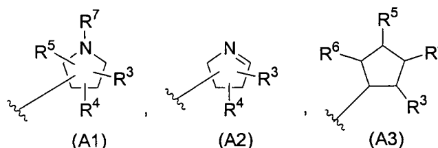
[Chemical formula 2]
