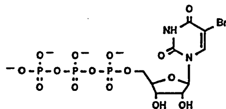
5-Bromo-UTP
