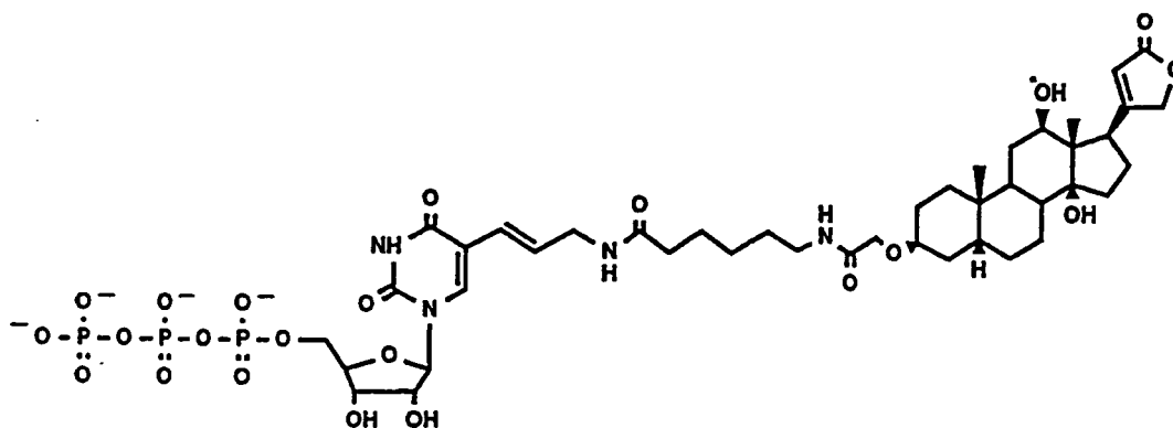
5-Digoxigenin-11-UTP
