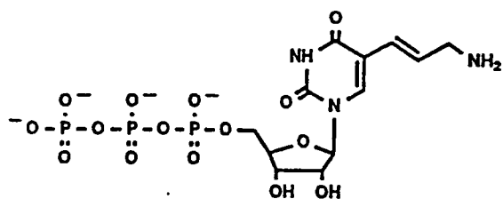
5-allylamino-UTP
