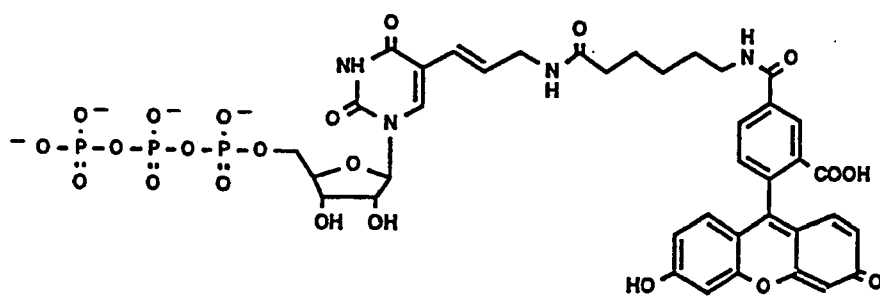
5-Fluorescein-12-UTP
