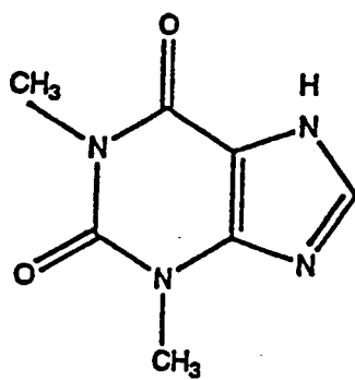
THEOPHYLLINE.
