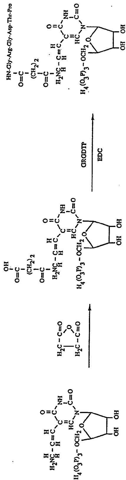
5-(3-Aminoallyl)-Uridine Triphosphate
