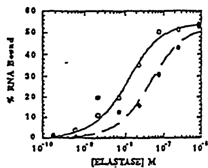
Binding with &amp; without KCl
