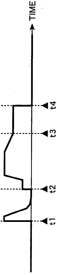
FIG. 10(E) CURRENT OF ELECTRO- MAGNETIC VALVE 105d
