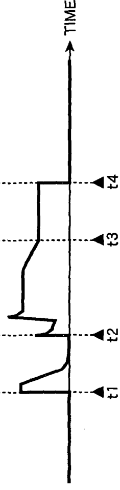
FIG. 15(E) CURRENT OF ELECTRO- MAGNETIC VALVE 105d
