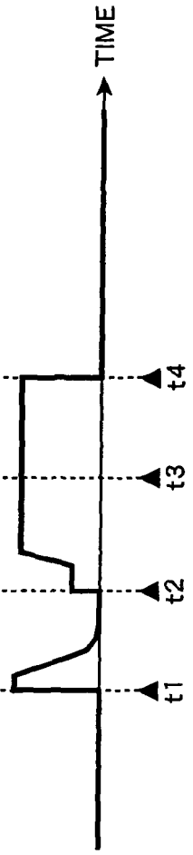
CURRENT OF ELECTRO- MAGNETIC VALVE 105d
