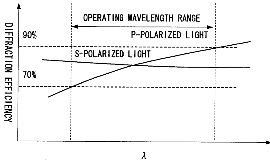
CHARACTERISTIC OF SINGLE DIFFRACTION GRATING
