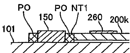
C-C CROSS SECTION
