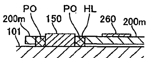
D-D CROSS SECTION
