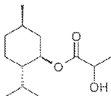
l-menthyl lactate
