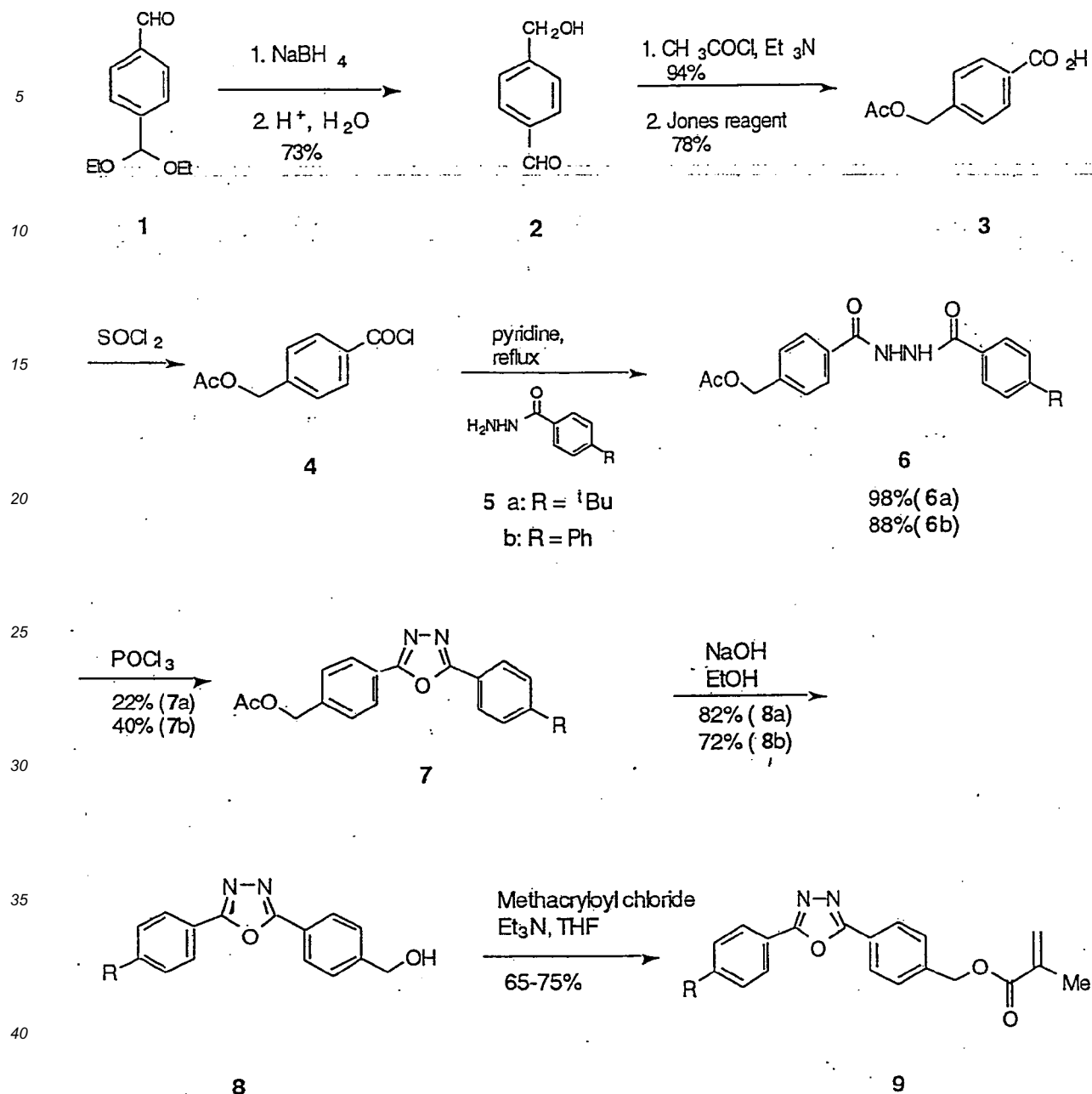
Scheme 5: Synthesis of oxadiazole monomers
