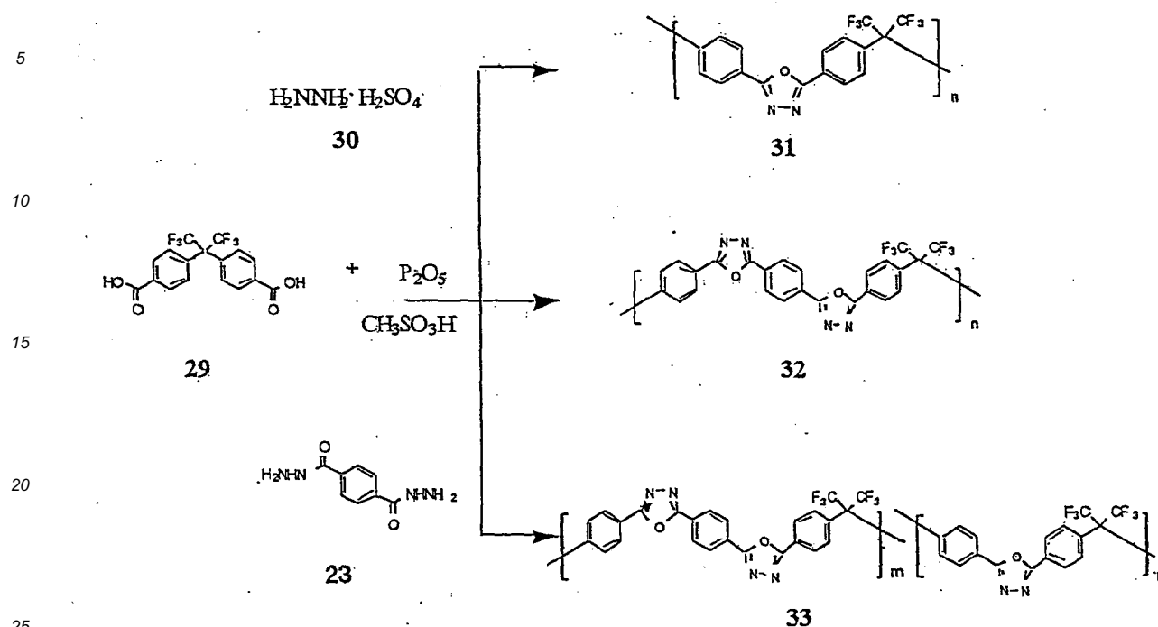
Scheme 10: The synthesis of fluorine-containing polyaromatic oxadiazoles
