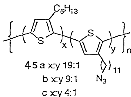
Figure 10 Representative polythiophenes for cross linking
