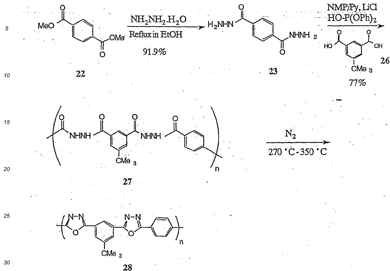
Scheme 9 : A Precursor route for the synthesis of a t Bu- aromatic oxadiazole polymer
