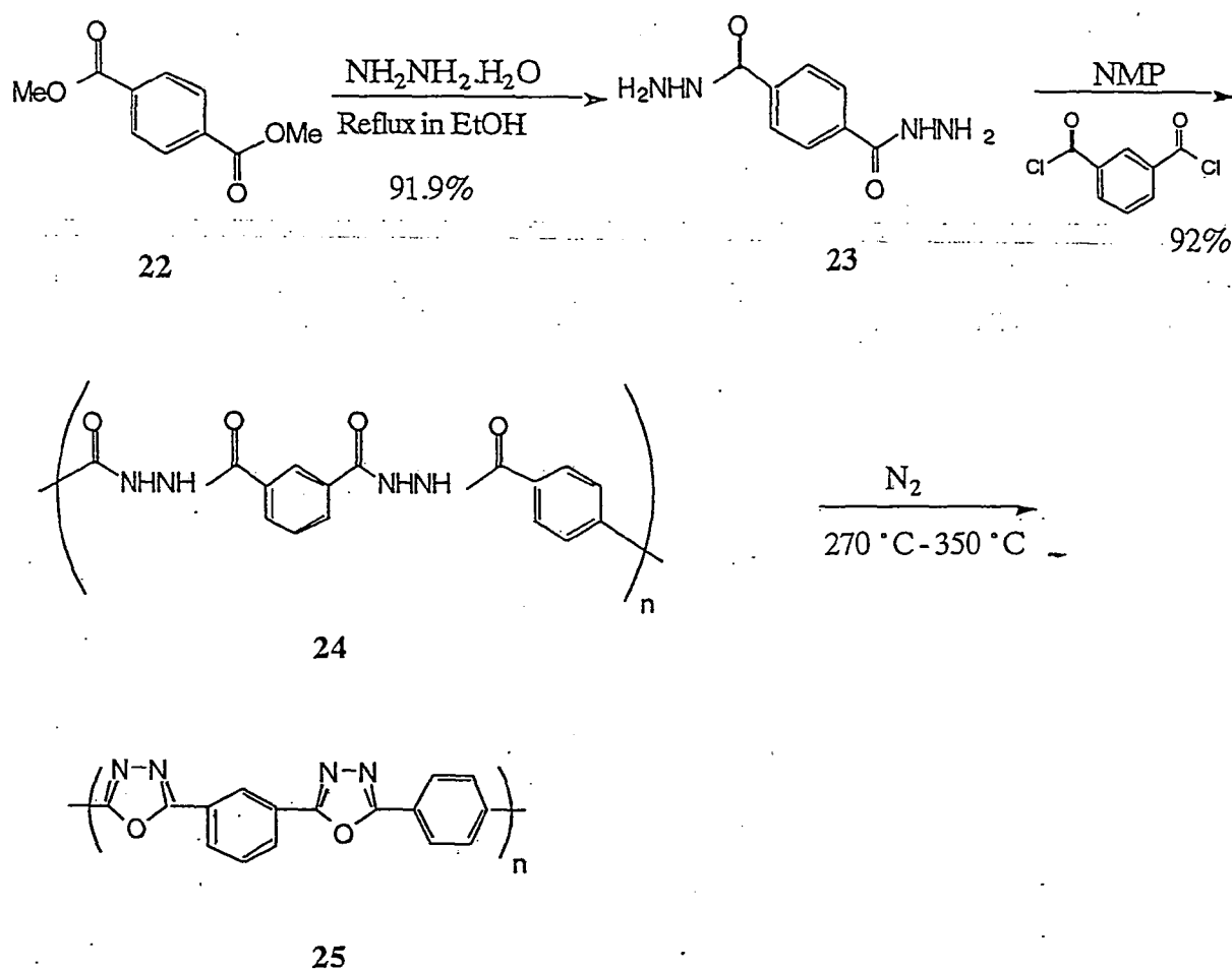
Scheme 8 : Precursor route for the synthesis of an aromatic oxadiazole polymer
