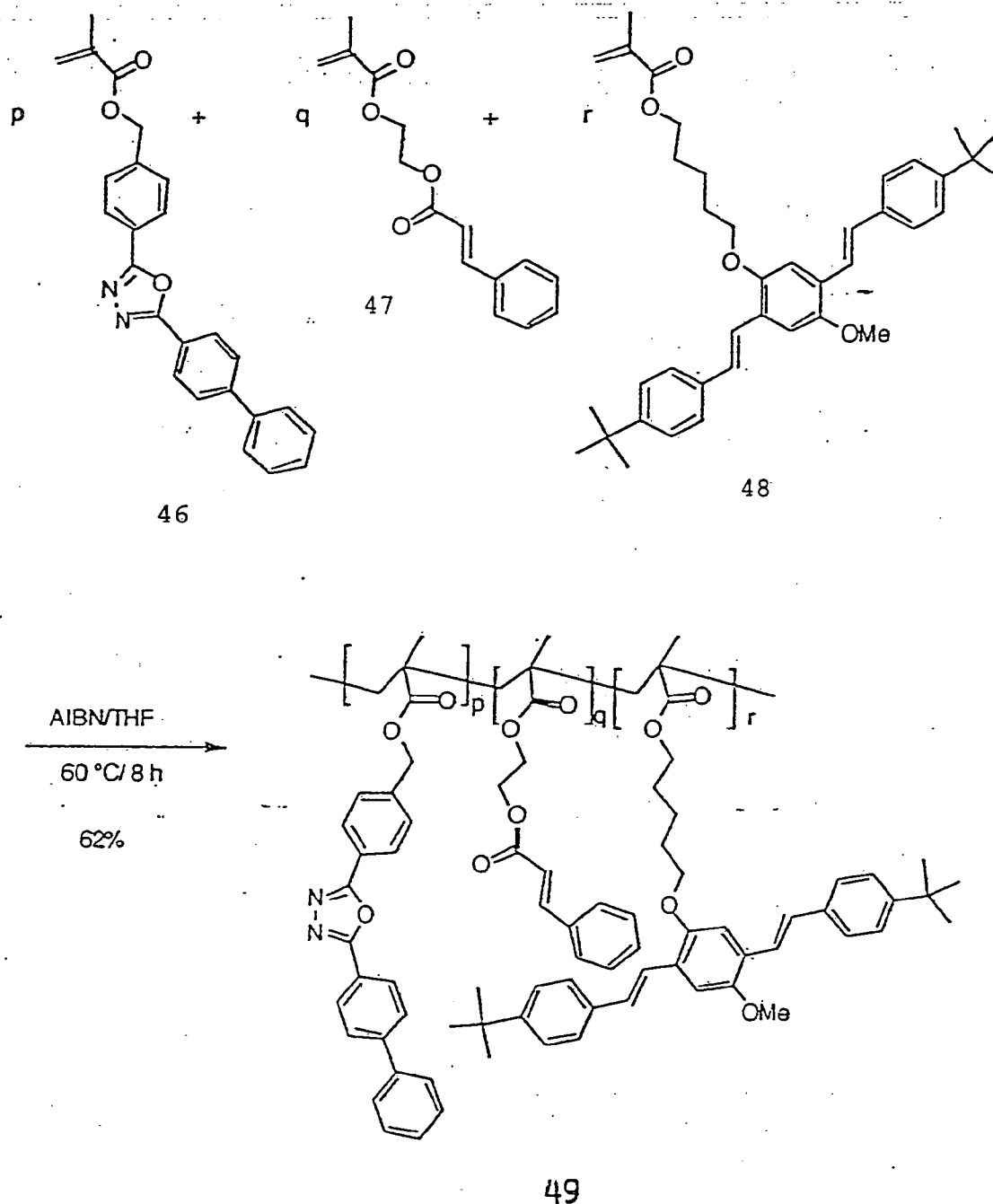
Scheme 12
