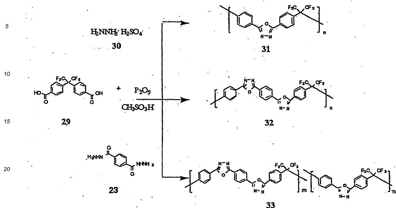
Scheme 10: The synthesis of fluorine-containing polyaromatic oxadiazoles
