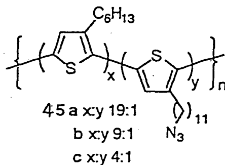
Figure 10 Representative polythiophenes for cross linking
