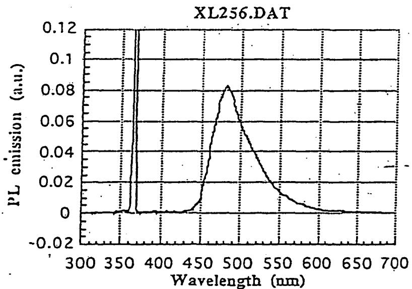
Figure 13: Photoluminescence spectrum of polymethacrylate 49 with 3 functional groups.
