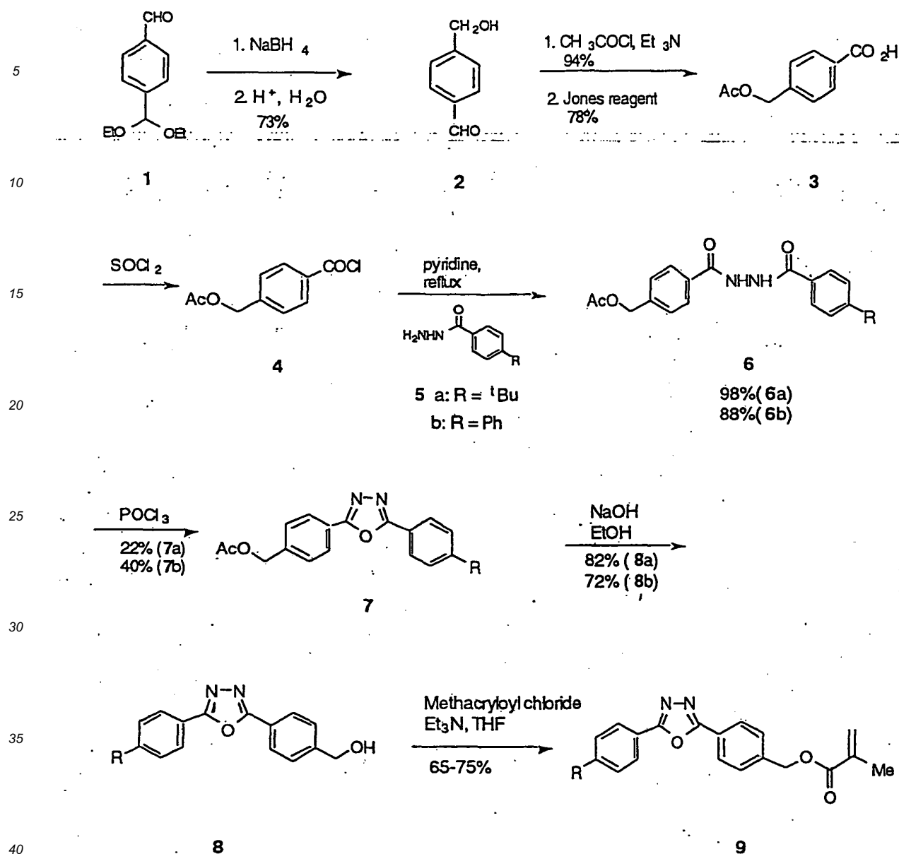
Scheme 5: Synthesis of oxadiazole monomers
