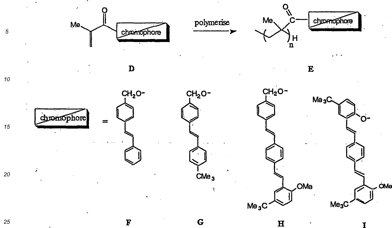
Scheme 6 A Poly(methacrylate) Containing a Blue Light Emitting Side Chain
