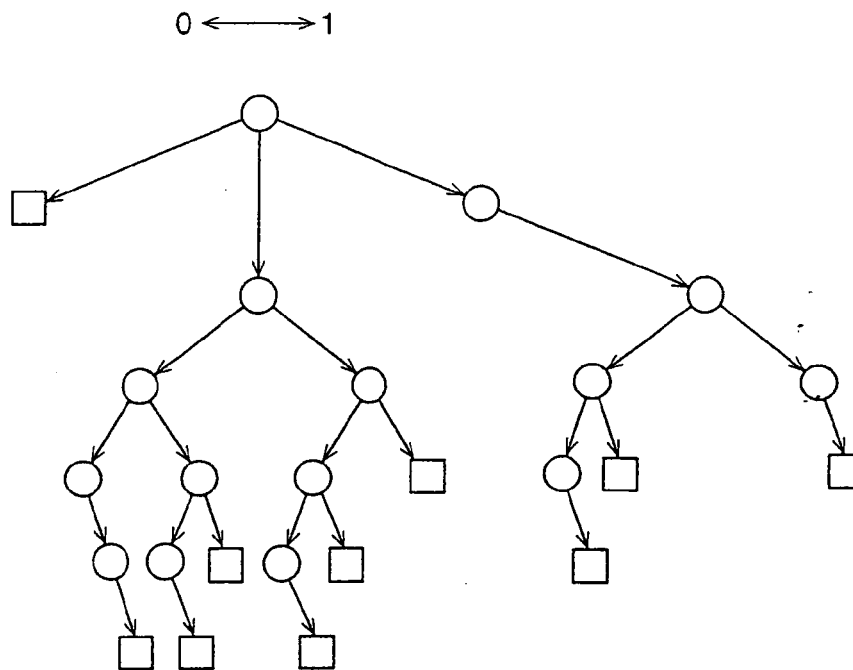
DECODING TREE
