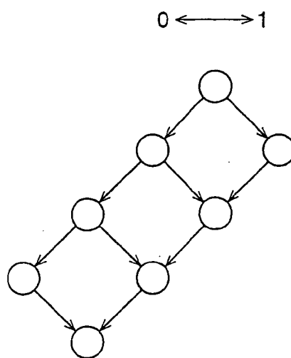
DECODING GRAPH
