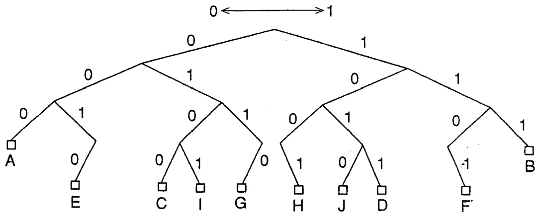
DECODING TREE IN ORDER DIRECTION
