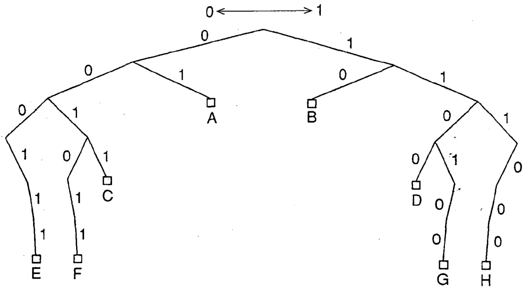
DECODING TREE IN ORDER DIRECTION
