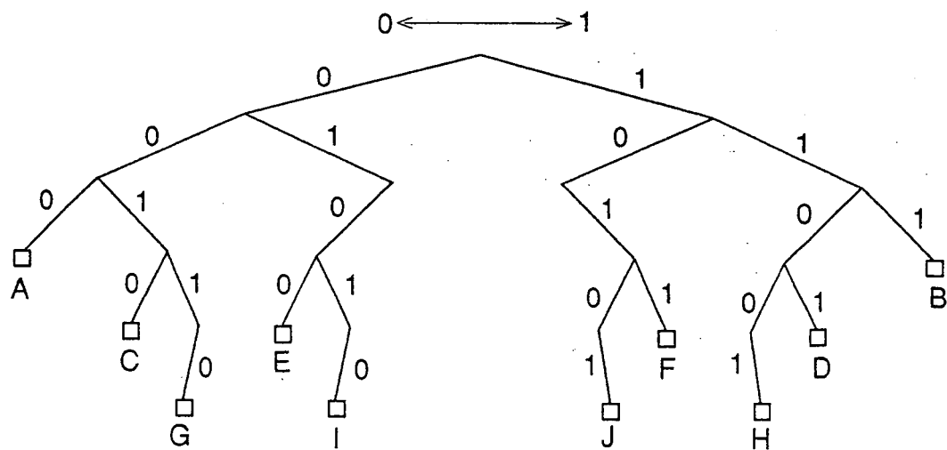
DECODING TREE IN REVERSE DIRECTION
