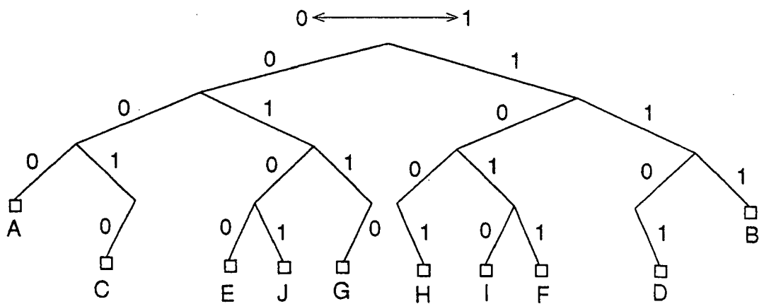
DECODING TREE IN REVERSE DIRECTION
