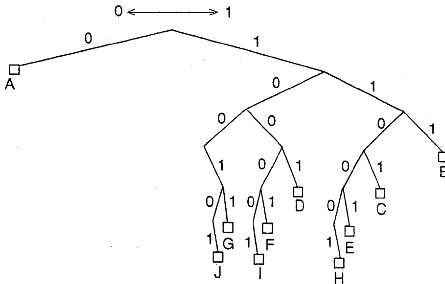
DECODING TREE IN REVERSE DIRECTION
