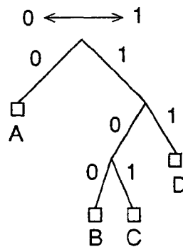
DECODING TREE IN ORDER DIRECTION
