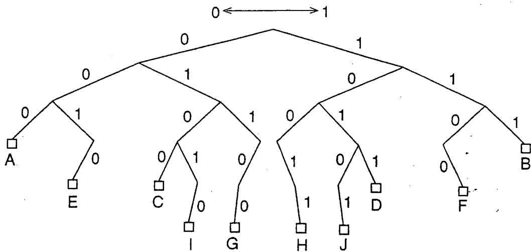
DECODING TREE IN THE ORDER DIRECTION
