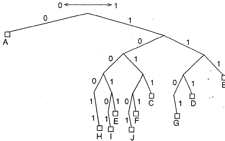
DECODING TREE IN THE ORDER
