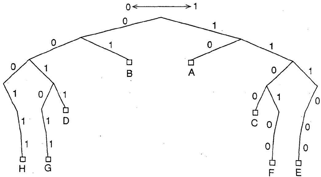
DECODING TREE IN REVERSE DIRECTION
