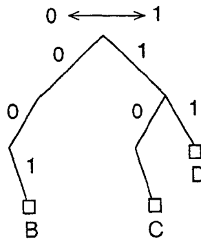
DECODING TREE IN REVERSE DIRECTION (IT IS IMPOSSIBLE TO CODE INSTANTANEOUSLY)
