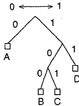
DECODING TREE IN ORDER DIRECTION
