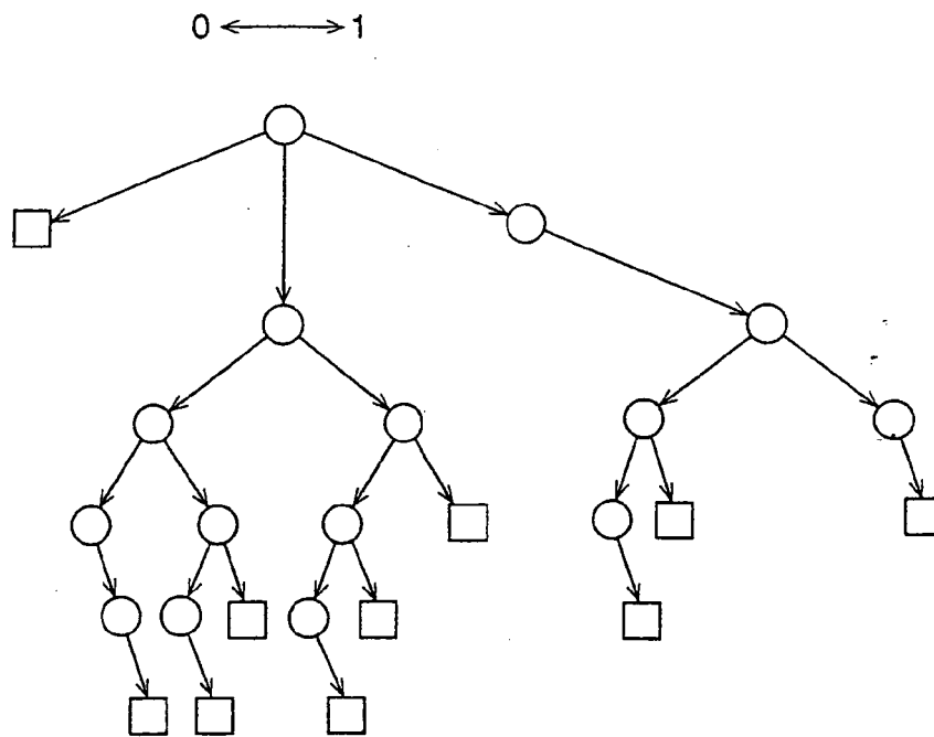
DECODING TREE
