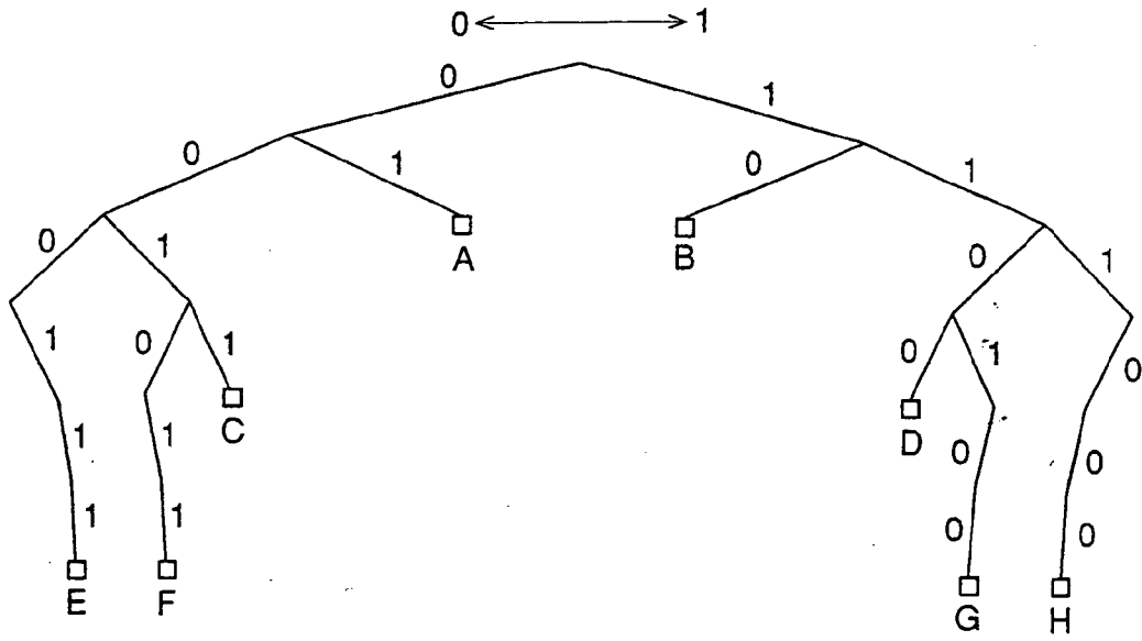
DECODING TREE IN ORDER DIRECTION
