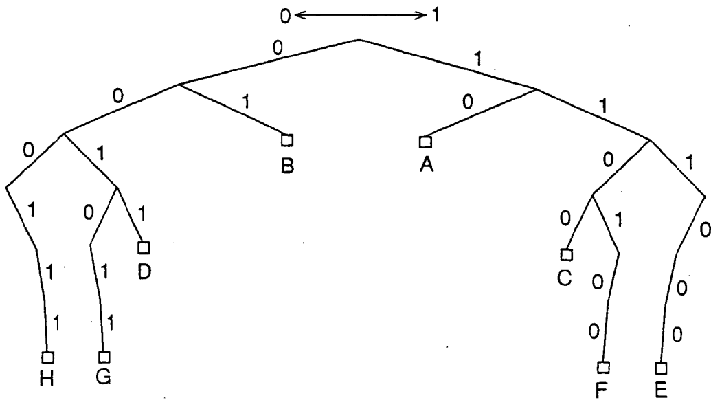
DECODING TREE IN REVERSE DIRECTION
