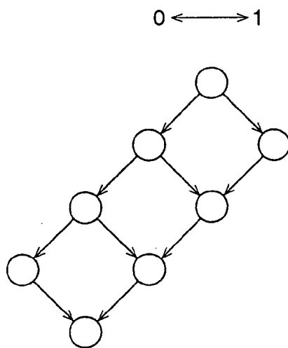
DECODING GRAPH
