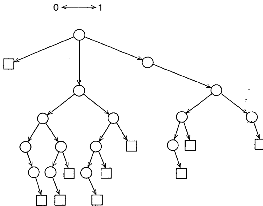
DECODING TREE
