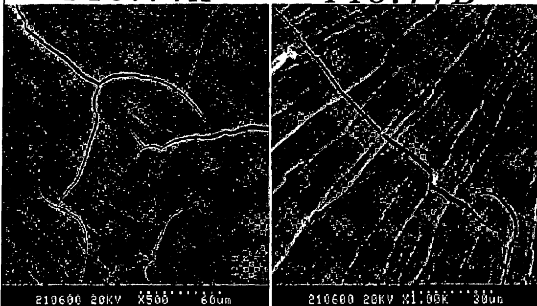
Cross-section of Solidified Super Glue with 16.2% PEG600, After Extraction by Water
