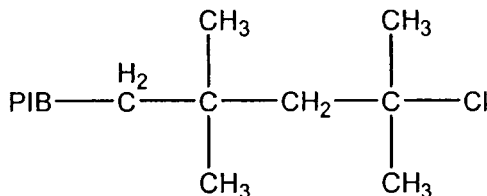
PIB tert-Chloride
