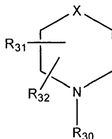
Formula IV
