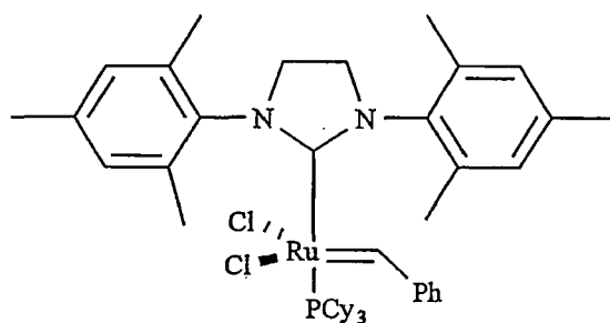
Grubbs Catalyst 3
