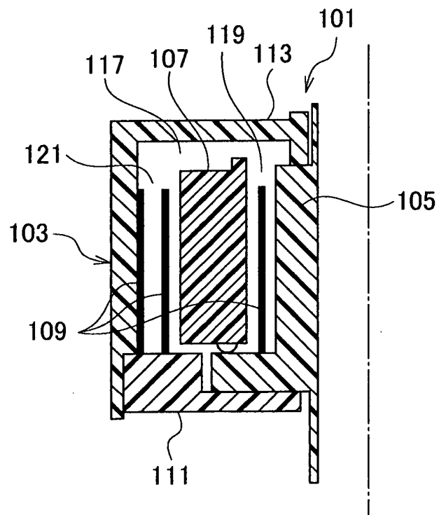
Fig.8 RELATED ART
