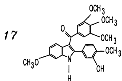
3-(3', 4', 5'-trimethoxy benzoyl) -2-(4'-methoxy - 5' hydroxy phenyl) -6-methoxy indole
