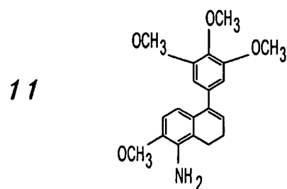
Amino dihydronaphthalene analog
