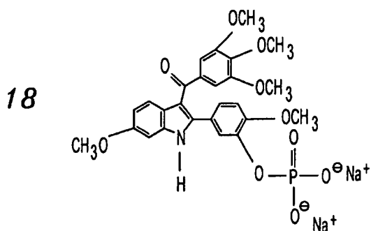
Indole sodium phosphate prodrug
