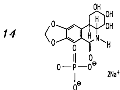
Pancratistatin sodium phosphate prodrug
