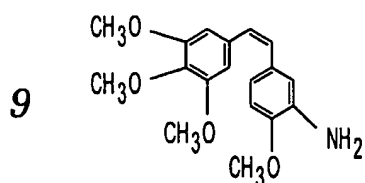
Amino Combretastatin A4 1-(3 amino -4 - methoxy phenyl) 2- (3,4,5 - tri methoxy phenyl) - ethene
