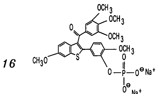
VPM-W-152 benzo(b)thiophene sodium phosphate prodrug
