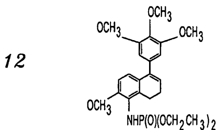
Amino dihydronaphthalene phosphoro amidate
