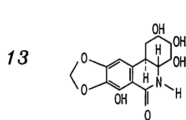
Amino dihydronaphthalene analog
