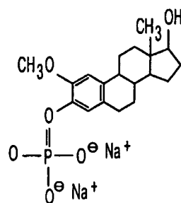
2-Methoxyestradiol sodium phosphate prodrug
