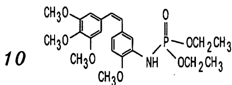
PM-VI-19C Amino Combretastatin A4 Phosphoro amidate prodrug
