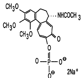
Colchicine sodium phosphate prodrug
