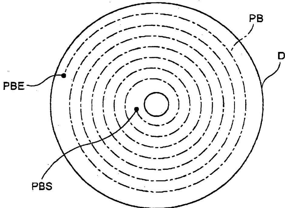
PREGROOVE VIEWED FROM THERMOSENSITIVE FACE
