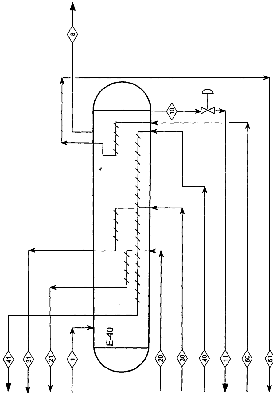
Figure 5 Alternate Embodiment Employing Only Cooling Water Utility
