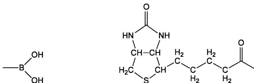
Boronic acid group
