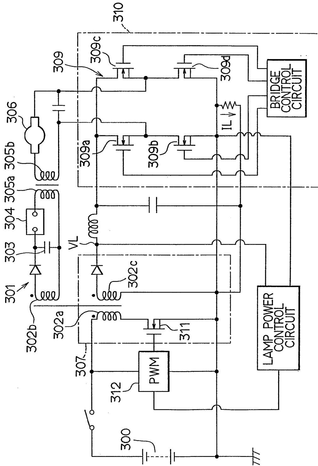
FIG. 26 RELATED ART
