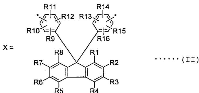
[Chem 13]
