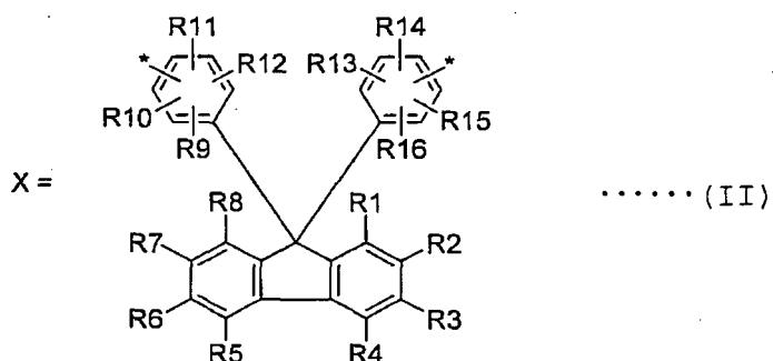
[Chem 2]
