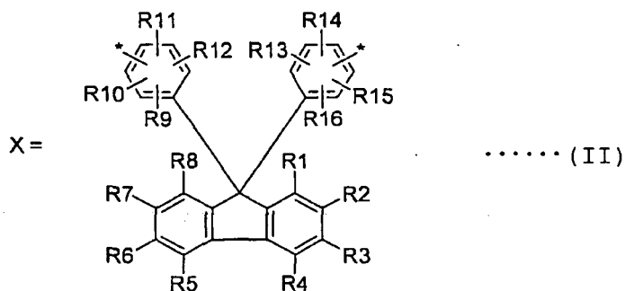
[Chem 4]
