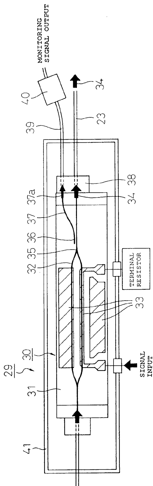
Fig.3 PRIOR ART
