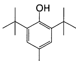
(R - 2 7)
