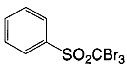
Polyhalogen compound-1
