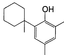
(R - 2 8)
