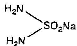
Reducing sensitizer C
