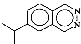
(Phthalazine compound-1C)
