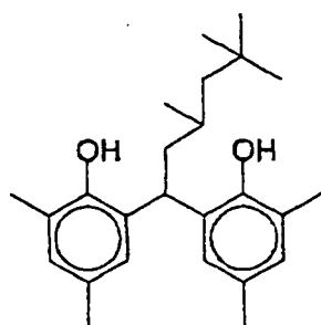
(Reducing agent-1e)
