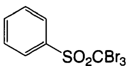
H-1
