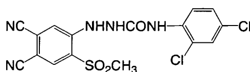
(A-3)
