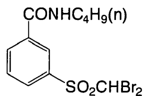
H-19
