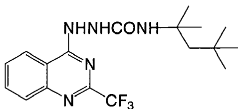
Development accelerator-1
