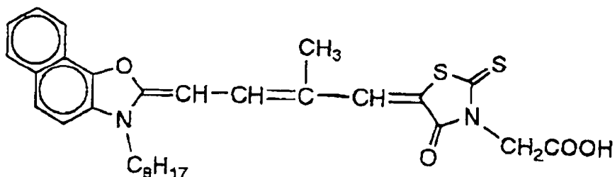
Spectral sensitizer B
