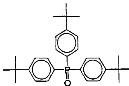
(Hydrogen coupling compound-2e)
