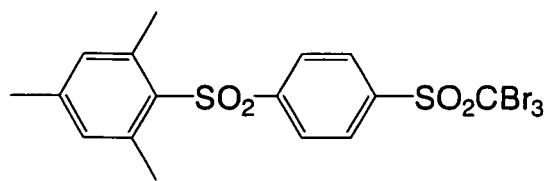
H-17
