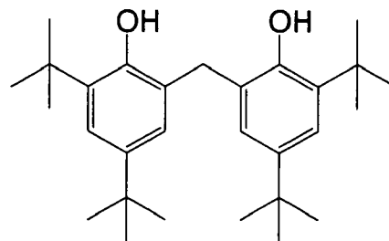
(R' - 12)
