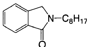
(D-20)
