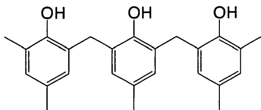
(R' - 19)
