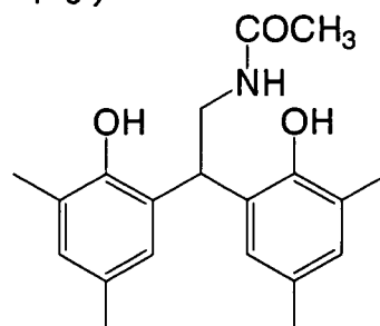
(R' ' - 1 6 )
