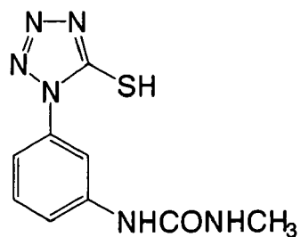
Mercapto compound-2
