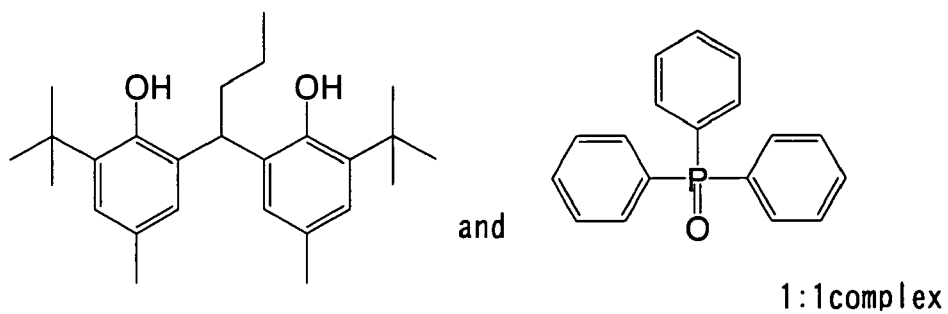
Reducing agent complex-1
