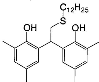
(R' - 19)
