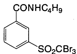
Polyhalogen compound-2
