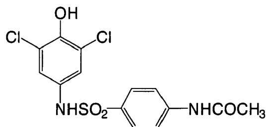
Development accelerator-2
