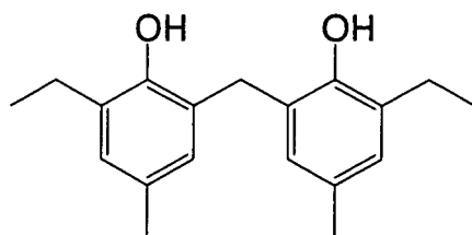
(R' - 7)
