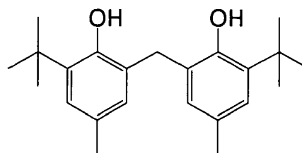
(R - 4)
