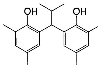
(R - 2)
