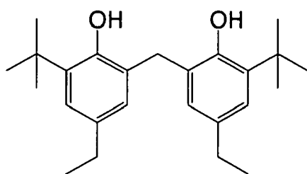
(R' - 9)
