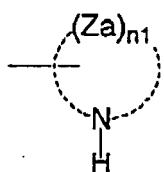
General Formula (X-2a)
