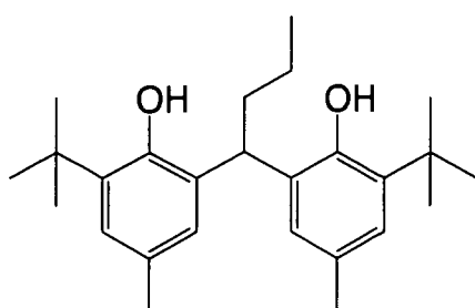
Reducing agent-1
