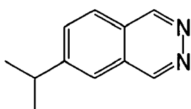
Phthalazine compound-1
