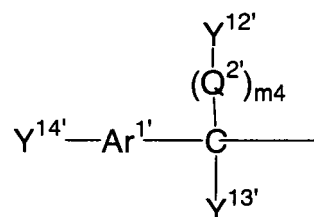
General Formula (A-2)
