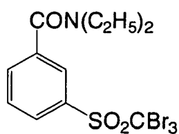
H-11
