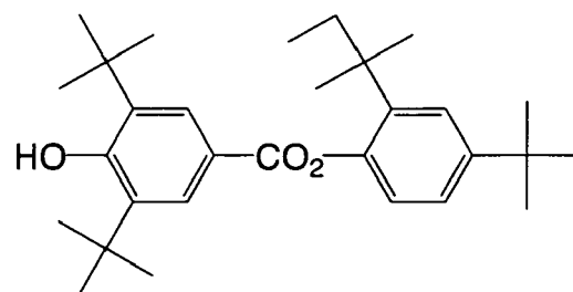
(R' - 30)
