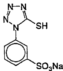
(Mercapto compound-1e)
