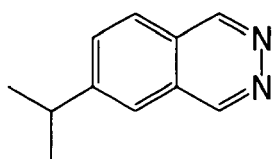
Phthalazine compound-1
