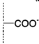
General Formula (B-1)
