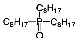
(D' - 7)
