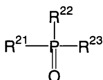
General Formula (D')
