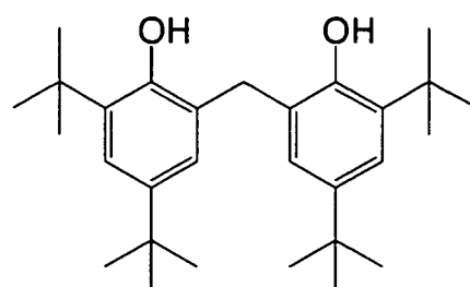
(R-10)
