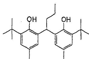
(Reducing agent-2)
