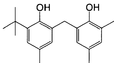
(R' ' - 1 1 )
