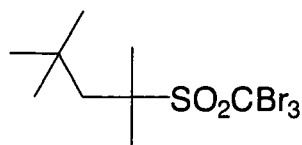
H-24
