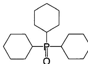
(D' - 6)
