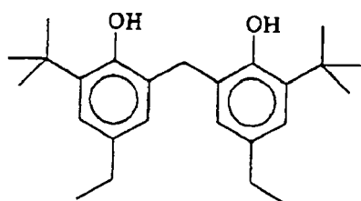
(Reducing agent-4C)
