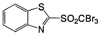
H-5
