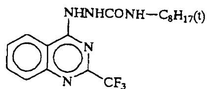
(Development accelerator 1C)
