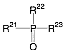
General Formula (D'')
