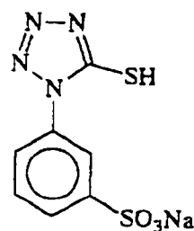
(Mercapto compound-1C)
