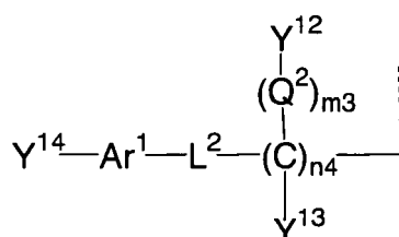
General Formula (A-1)
