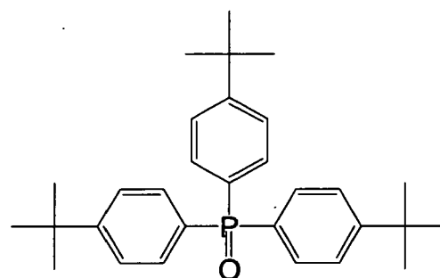
Hydrogen bonding type compound-1
