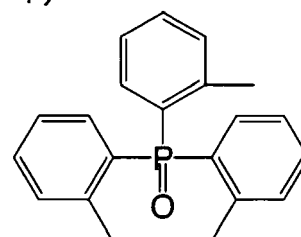
(D-4)
