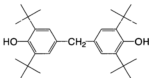
(R' - 3 2)
