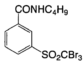
Polyhalogen compound-2
