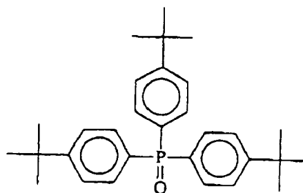
(Hydrogen coupling compound-2C)
