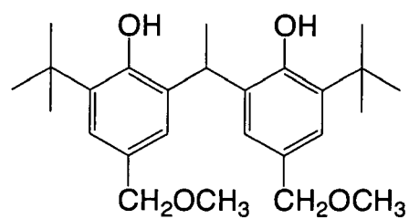
(R - 2 2)
