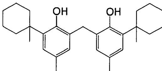
(R-17)
