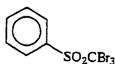
(Polyhalogen compound-2C)
