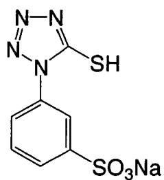
Mercapto compound-1
