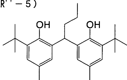
(R' - 5)
