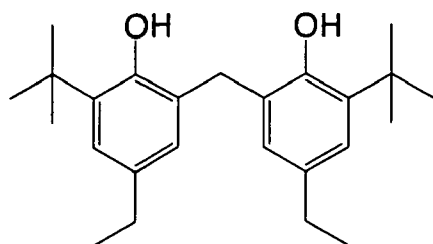
(R' - 9)
