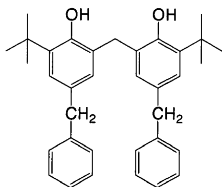
(R - 2 3)
