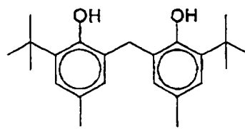
(Reducing agent-5e)
