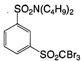
H-12
