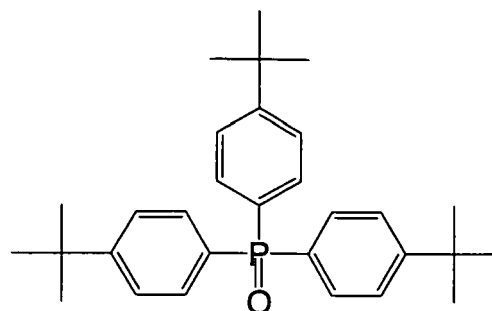
Hydrogen bonding type compound-1
