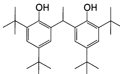
(R' - 8)
