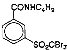
(Organic polyhalogen compound-3e)
