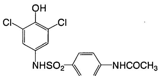
Development accelerator-2
