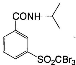
H-9
