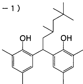
(R' - 3)
