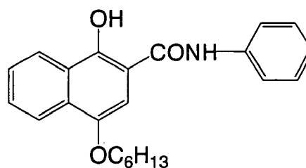
Development accelerator-3
