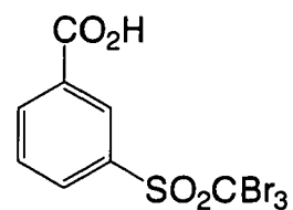
H-15
