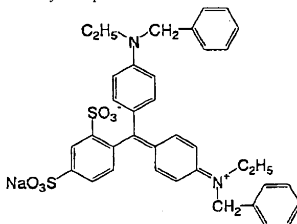
Blue dye compound 14
