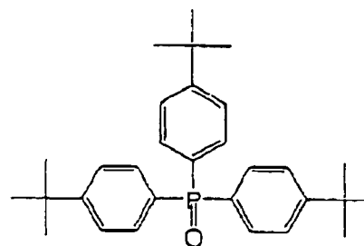
(Hydrogen coupling compound-1)
