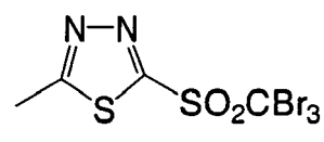
H-6
