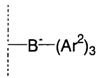
General Formula (B-3)
