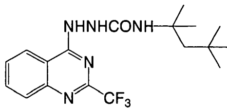
Development accelerator-1
