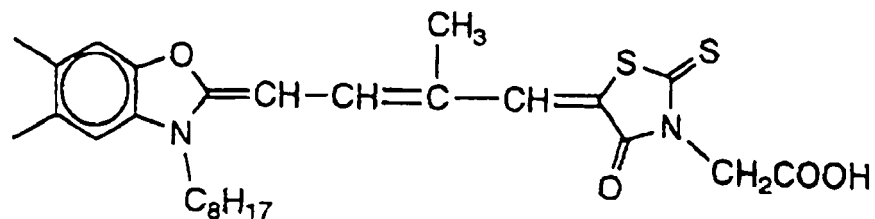
Spectral sensitizer A
