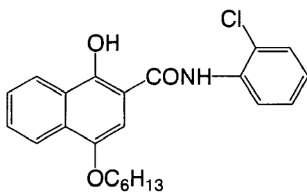
Development accelerator-2'
