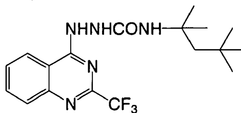
Development accelerator-1
