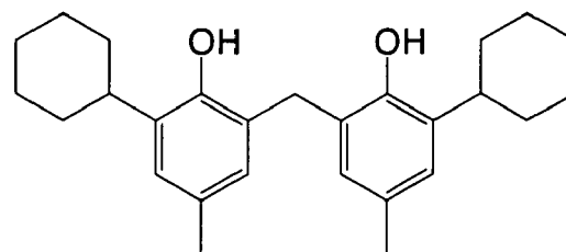
(R-16)
