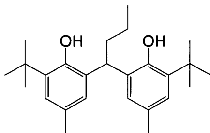
Reducing agent-2
