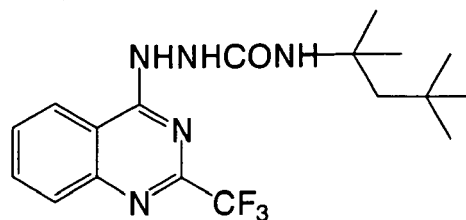
Development accelerator-1
