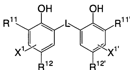
General Formula (R'')
