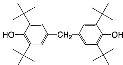
Color tone adjusting agent-1
