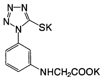
Chemical formula (1-2)
