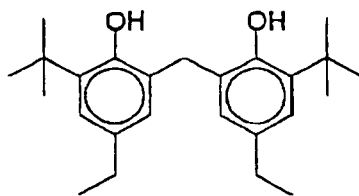
(Reducing agent-4e)
