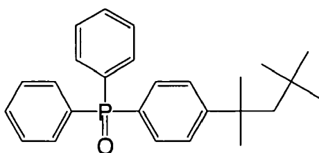
(D-17)
