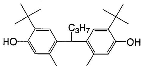
(R' - 3 3)
