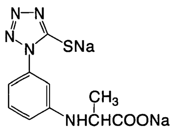
Chemical formula (1-1)
