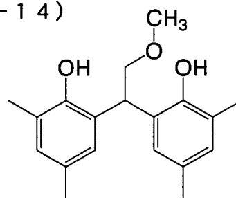
(R' ' - 1 6 )
