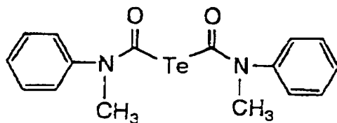
Tellurium sensitizer C
