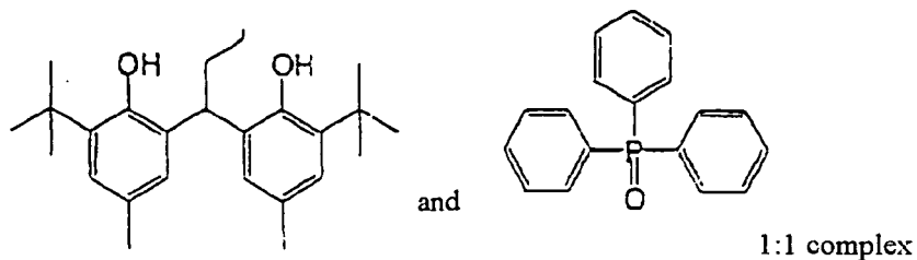
(Reducing agent complex-1)
