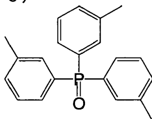
(D-3)
