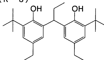
(R-8)
