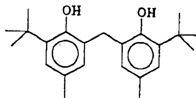
(Reducing agent-5C)
