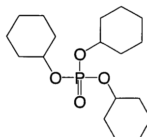
(D' - 8)
