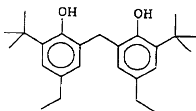
(Reducing agent complex-3C)
