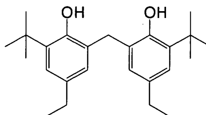
(R' - 6)
