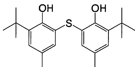
(R - 2 5)
