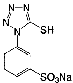
Mercapto compound-1
