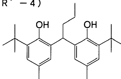
(R' - 4)
