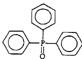
(Hydrogen coupling compound-1C)
