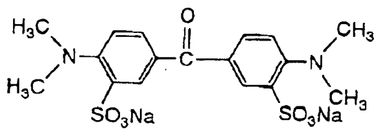
Yellow dye compound 15
