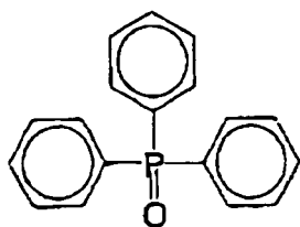
(Hydrogen coupling compound-1e)
