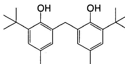
Reducing agent-3'
