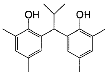
Reducing agent-2'
