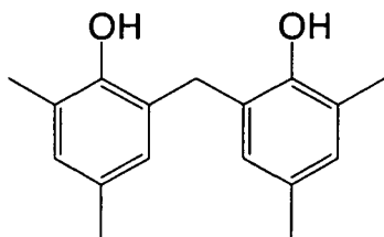
(R' - 3)
