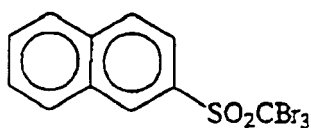
(Polyhalogen compound-1C)
