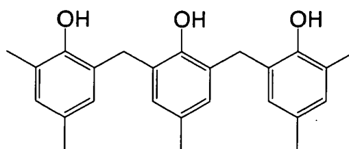
(R - 2 4)
