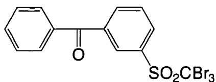
H-18
