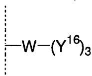
General Formula (B-2)
