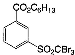
H-13
