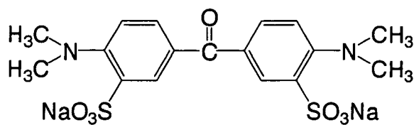
Yellow dye compound-1
