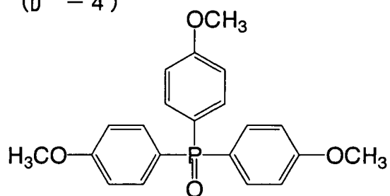
(D' - 4)
