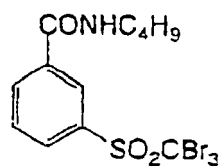
(Polyhalogen compound-2)
