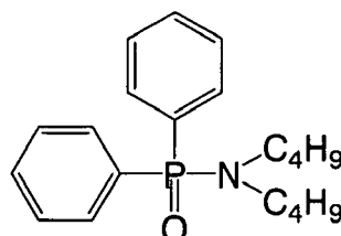
(D-16)
