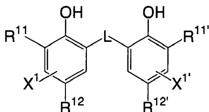
General Formula (R)
