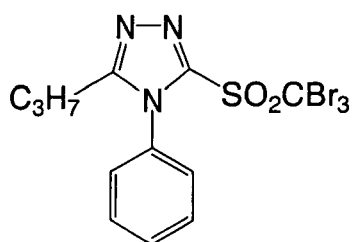
H-10
