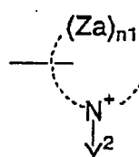
General Formula (X-2b)
