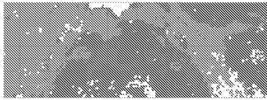
Raman map
