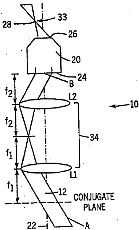
FIG. 2 PRIOR ART
