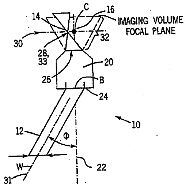
FIG. 1 PRIOR ART
