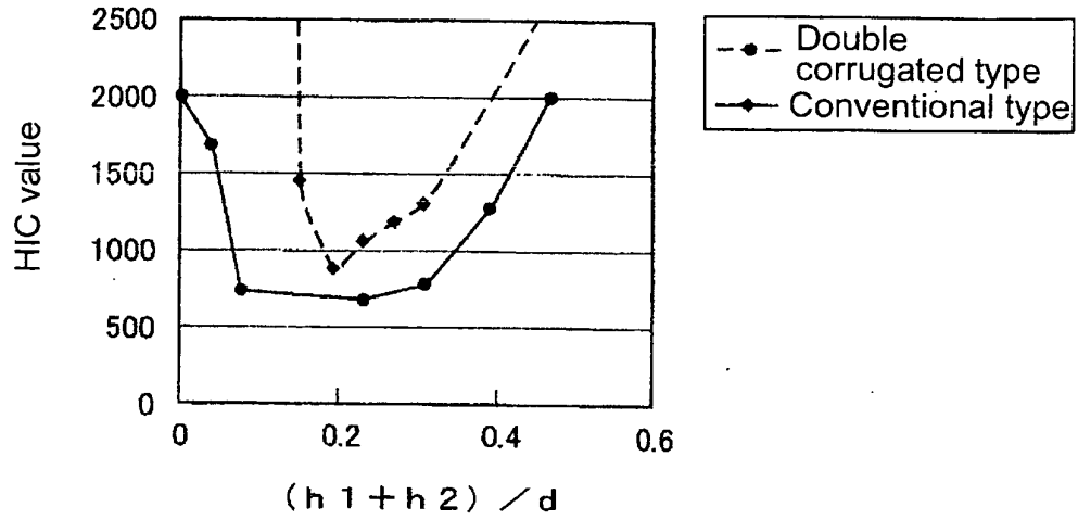
Relationship between wave height and HIC value (clearance 70mm, wave height 165mm)
