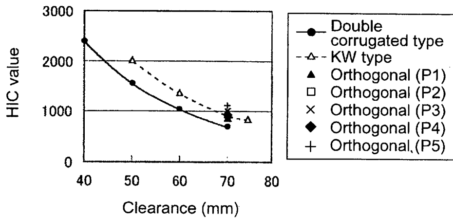
Relationship between clearance and HIC value (wave length 165mm, wave height (h1+h2)=30mm)
